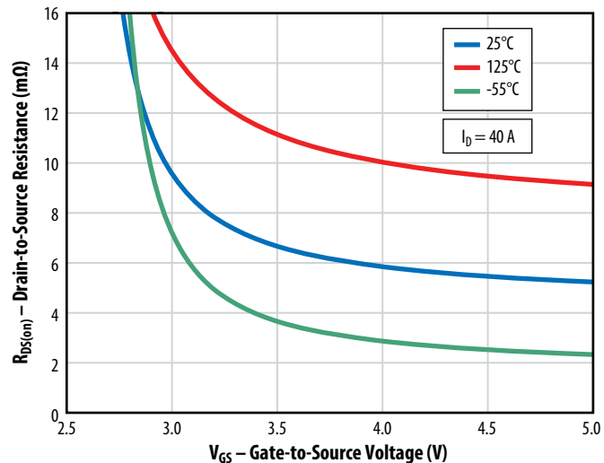
Figure 5: R_{DS(on)} vs. V_{GS} for Various Temperatures
