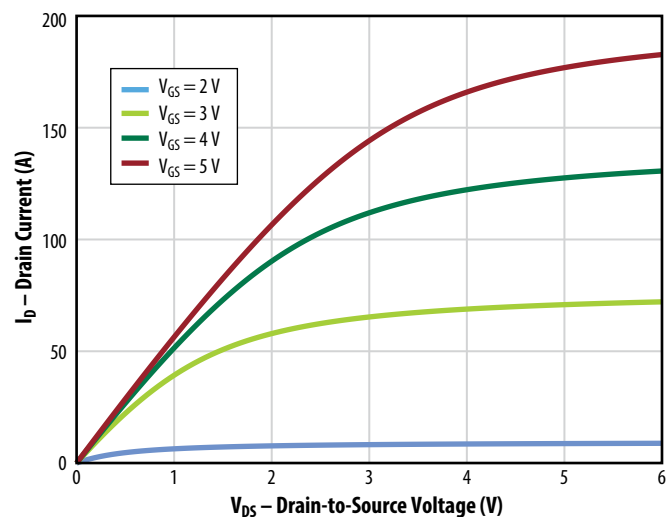
Figure 3: Typical Output Characteristics at 125°C
