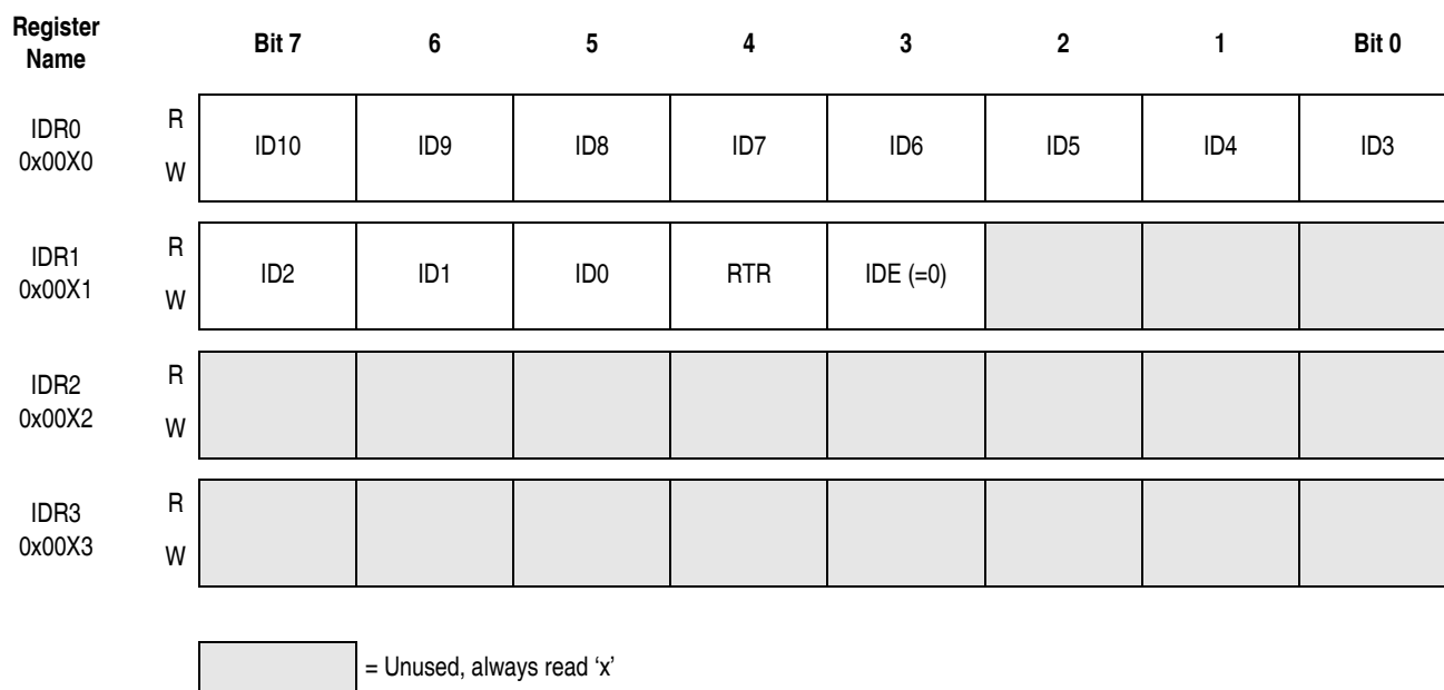
Figure 13-24. Receive/Transmit Message Buffer — Standard Identifier Mapping
