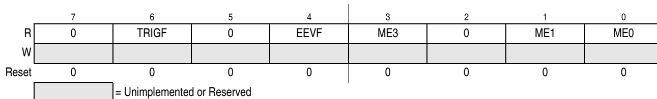
Figure 7-9. Debug Event Flag Register (DBGEFR)
