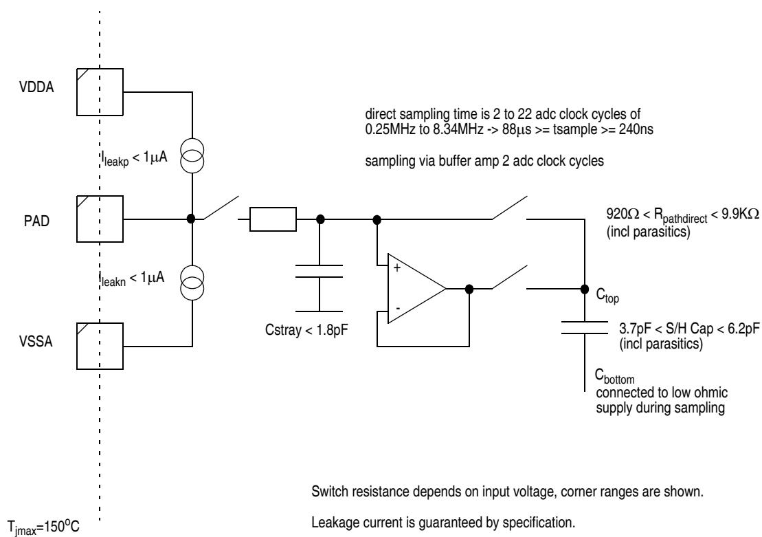
Figure C-1. ADC input logic
