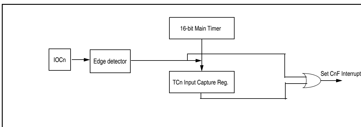
Figure 16-2. Interrupt Flag Setting
