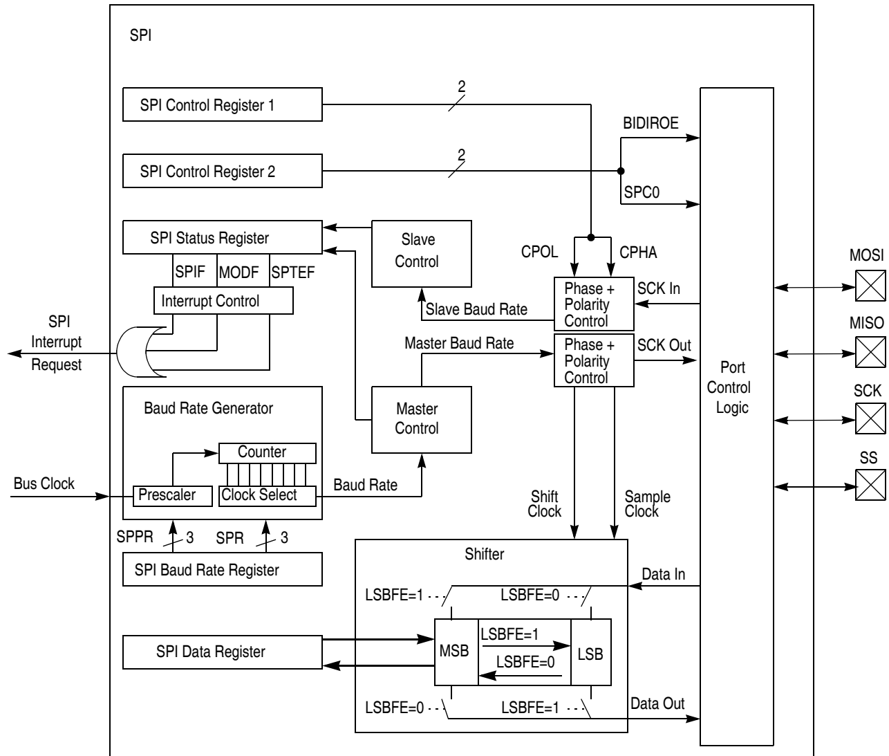
Figure 19-1. SPI Block Diagram
