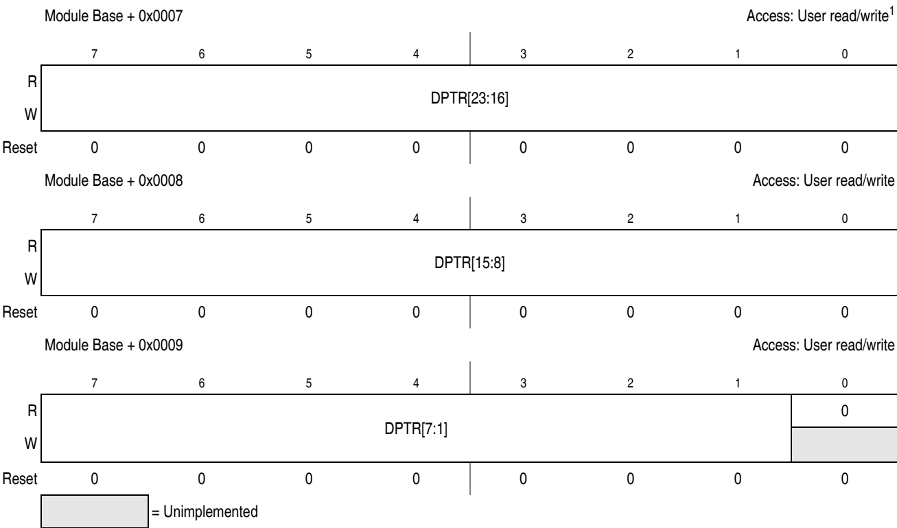
Figure 8-5. ECC Debug Pointer Register (ECCDPTRH, ECCDPTRM, ECCDPTRL)
