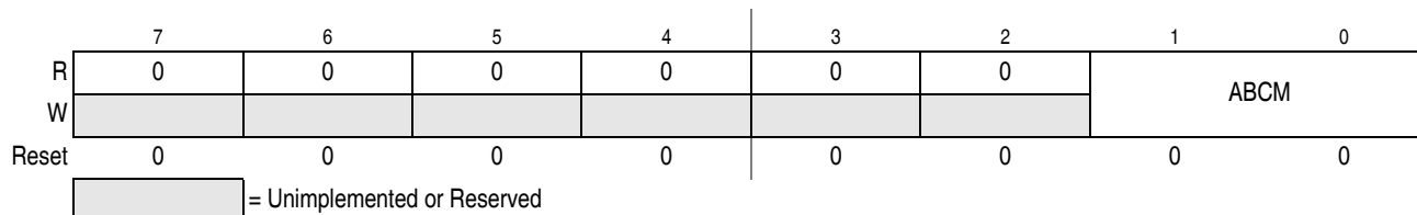
Figure 7-4. Debug Control Register2 (DBG2)
