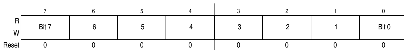
Figure 17-11. PWM Scale B Register (PWMSCLB)
