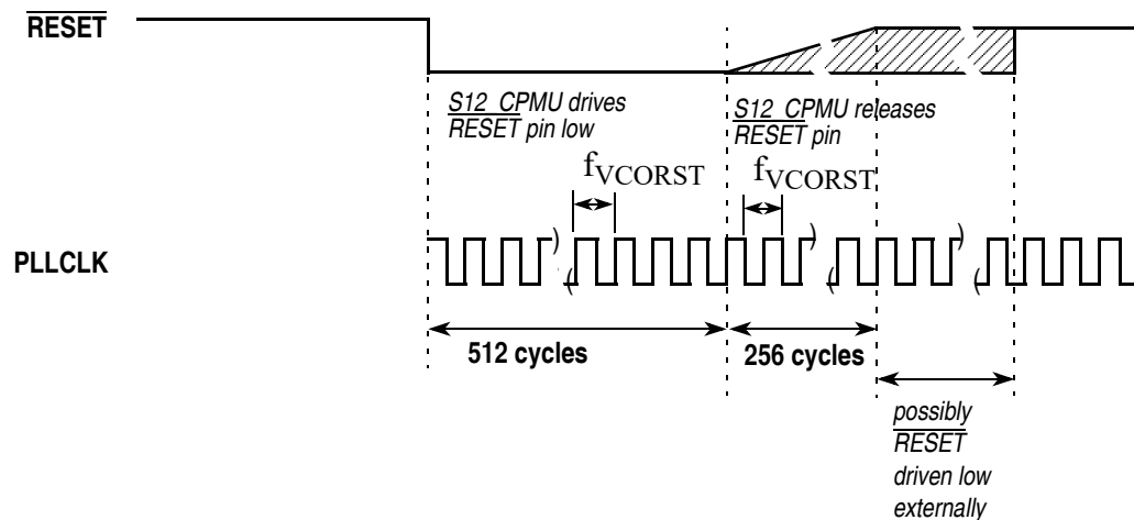
Figure 9-42. RESET Timing
