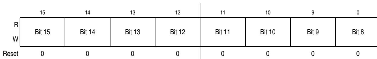
Figure 15-18. Timer Input Capture/Output Compare Register x High (TCxH)
