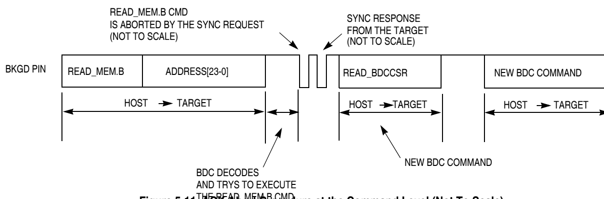
Figure 5-11. ACK Abort Procedure at the Command Level (Not To Scale)
