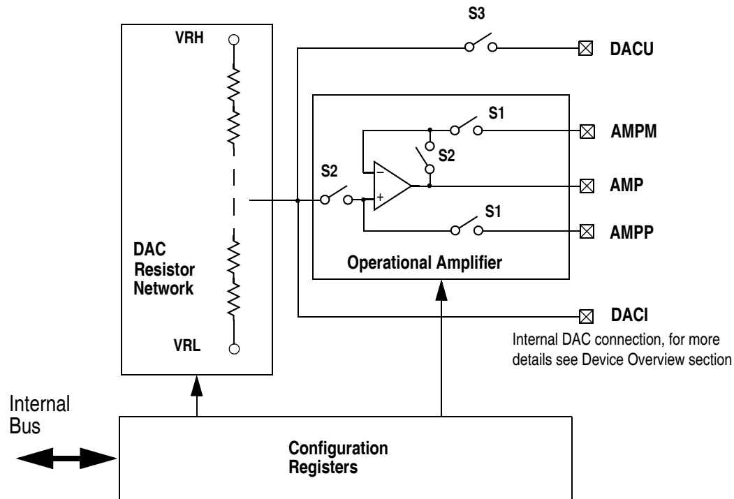
Figure 11-1. DAC_8B5V Block Diagram
