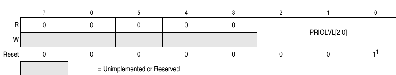
Figure 6-11. Interrupt Request Configuration Data Register 6 (INT_CFDATA6)
