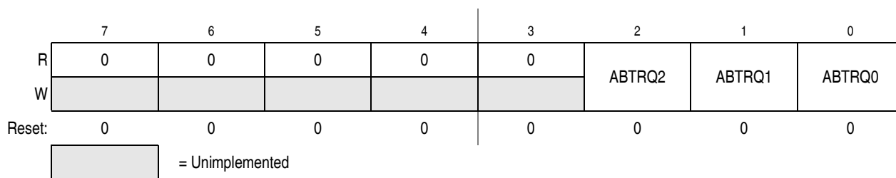
Figure 13-12. MSCAN Transmitter Message Abort Request Register (CANTARQ)
