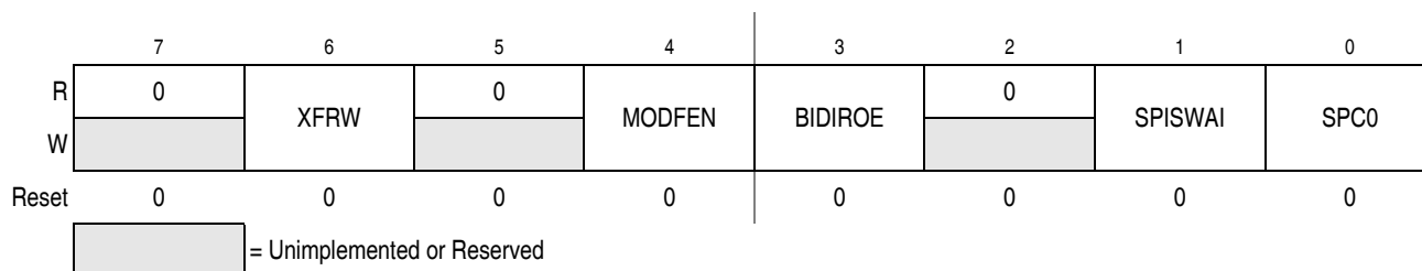
Figure 19-4. SPI Control Register 2 (SPICR2)
