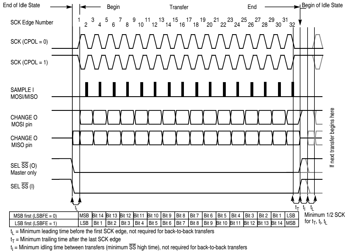
Figure 19-15. SPI Clock Format 1 (CPHA = 1), with 16-Bit Transfer Width selected (XFRW = 1)
