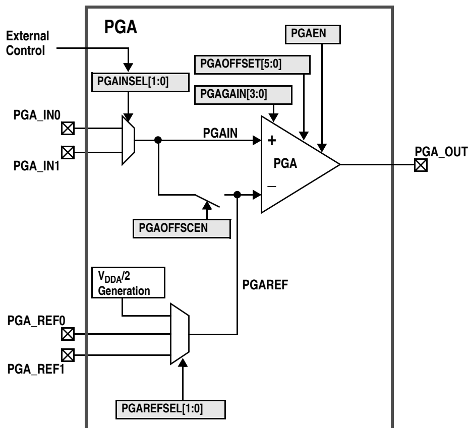
Figure 12-1. PGA Block Diagram
