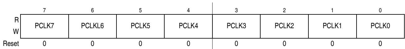
Figure 17-5. PWM Clock Select Register (PWMCLK)
