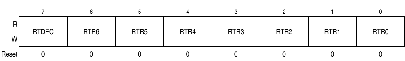
Figure 9-14. S12CPMU_UHV RTI Control Register (CPMURTI)
