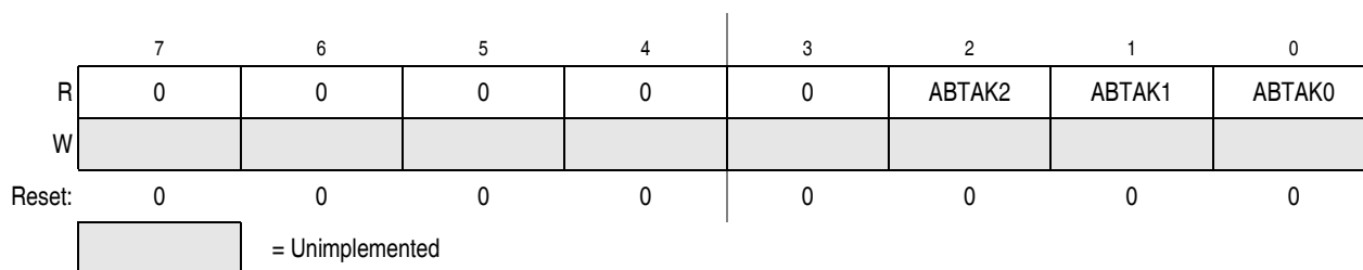
Figure 13-13. MSCAN Transmitter Message Abort Acknowledge Register (CANTAACK)
