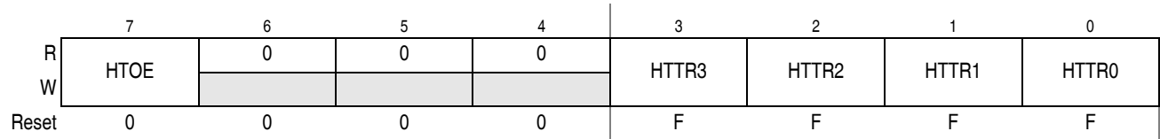
Figure 9-28. High Temperature Trimming Register (CPMUHTTR)
