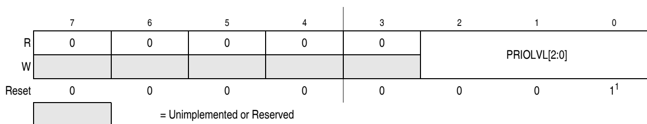
Figure 6-9. Interrupt Request Configuration Data Register 4 (INT_CFDATA4)
