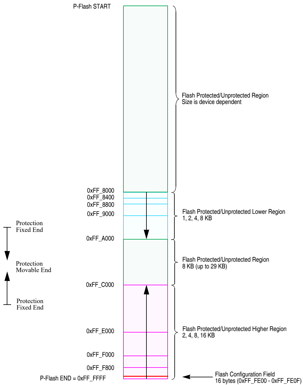
Figure 22-2. P-Flash Memory Map With Protection Alignment
