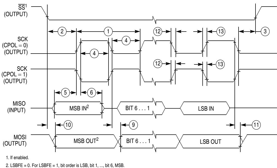
Figure K-1. SPI Master Timing (CPHA=0)
