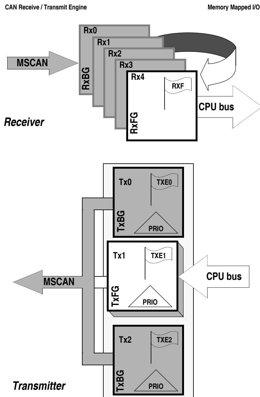
Figure 13-38. User Model for Message Buffer Organization
