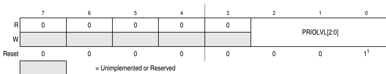
Figure 6-7. Interrupt Request Configuration Data Register 2 (INT_CFDATA2)
