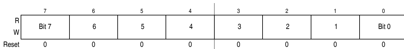
Figure 17-10. PWM Scale A Register (PWMSCLA)
