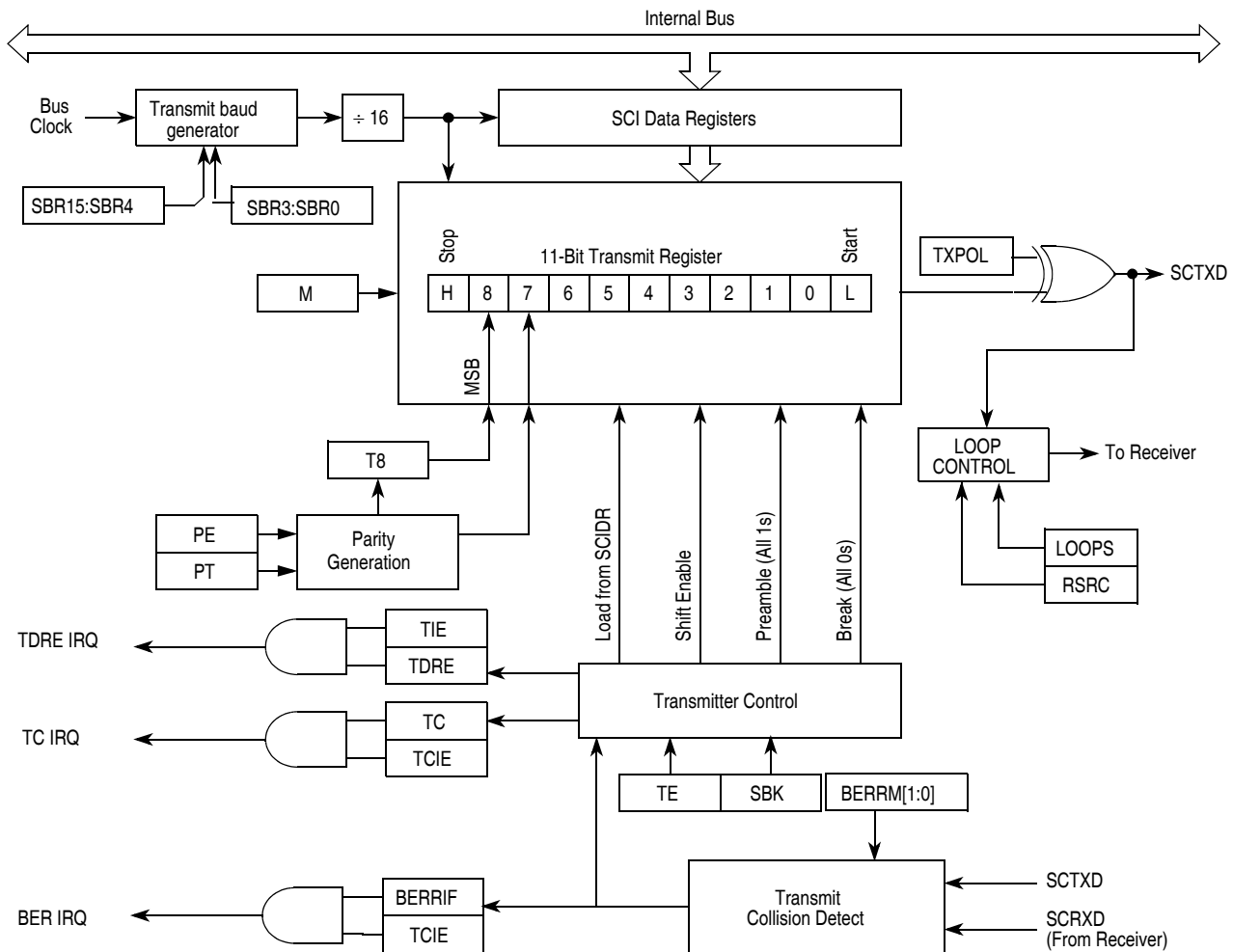
Figure 18-16. Transmitter Block Diagram
