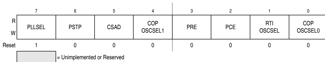
Figure 9-12. S12CPMU_UHV Clock Select Register (CPMUCLKS)
