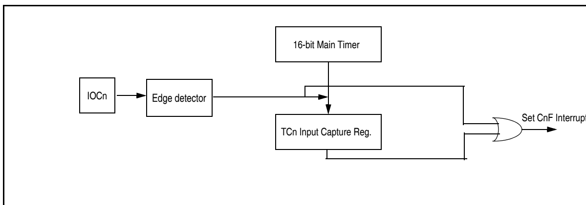
Figure 15-2. Interrupt Flag Setting
