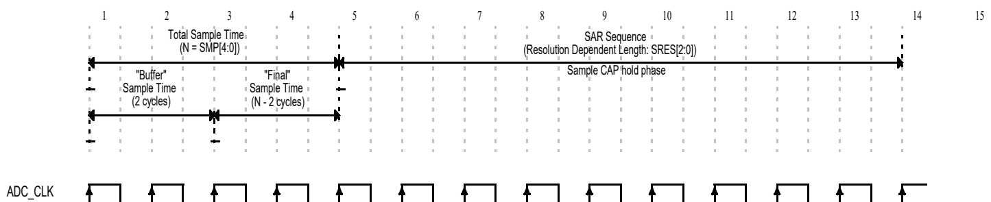
Figure 10-28. Sampling and Conversion Timing Example (8-bit Resolution, 4 Cycle Sampling)
