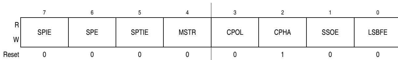
Figure 19-3. SPI Control Register 1 (SPICR1)
