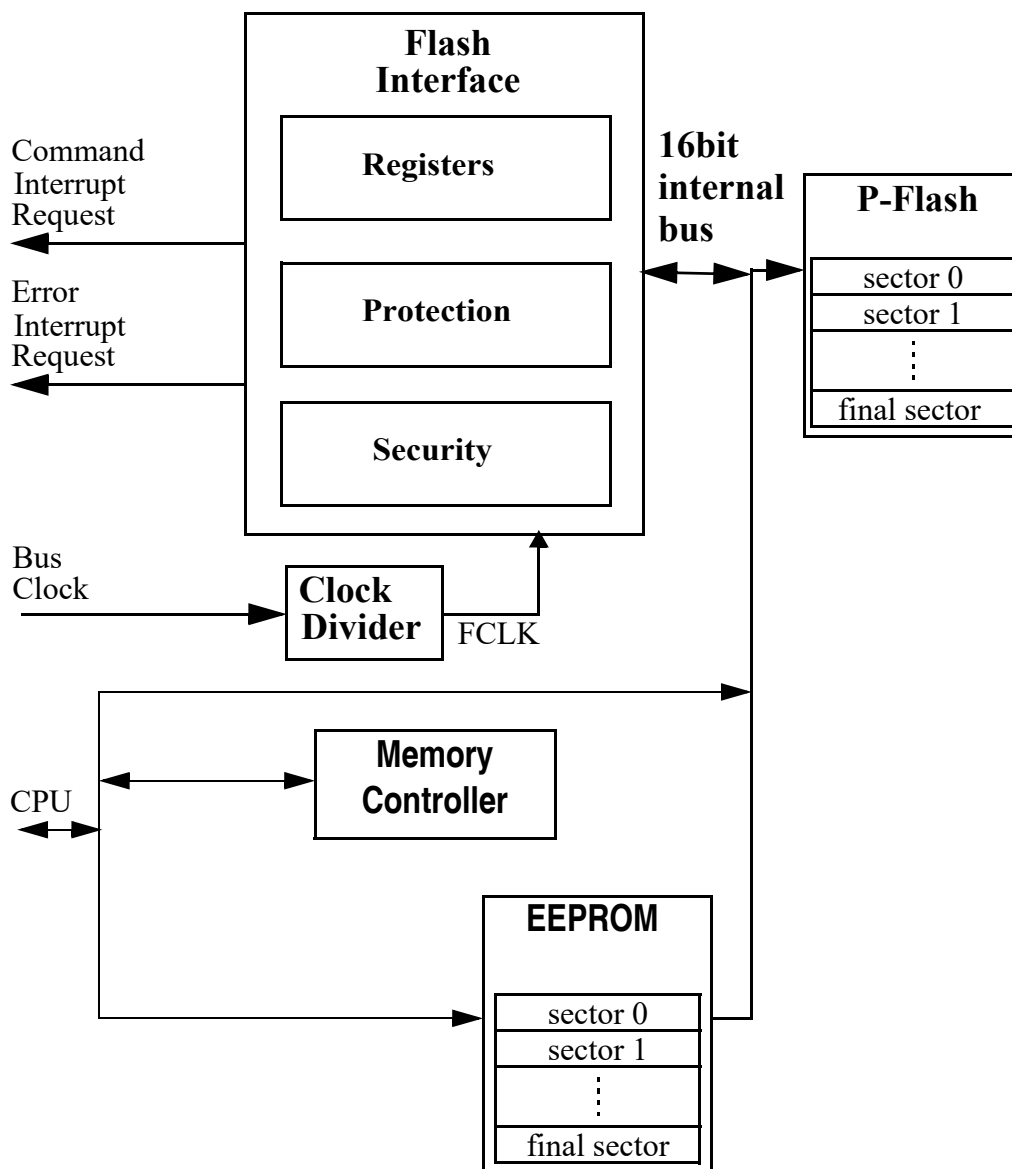
Figure 22-1. FTMZRZ Block Diagram
