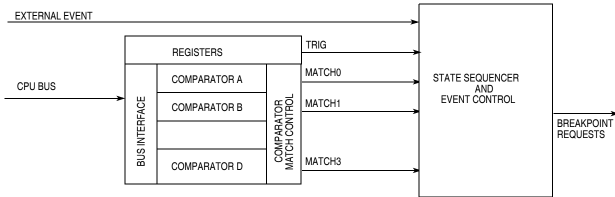
Figure 7-1. Debug Module Block Diagram
