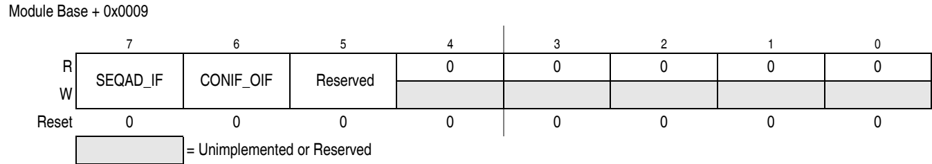
Figure 10-13. ADC Interrupt Flag Register (ADCIF)
