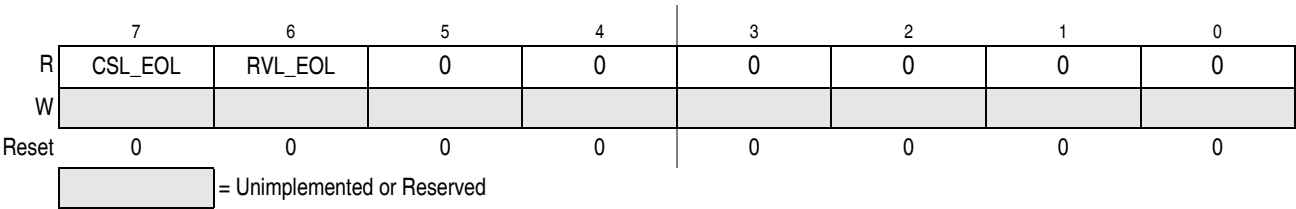
Figure 10-17. ADC End Of List Result Information Register (ADCEOLRI)
