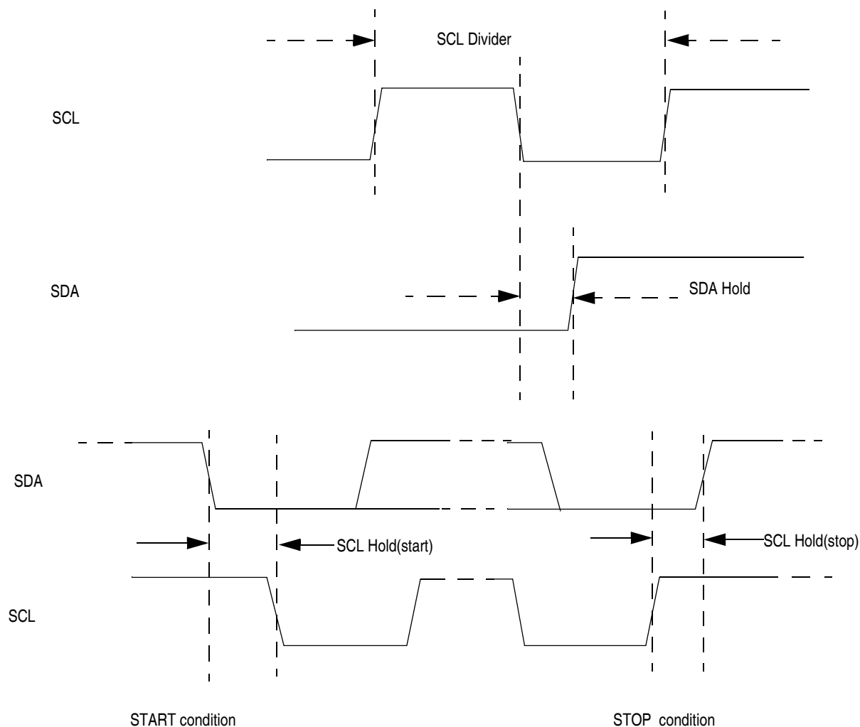
Figure 20-5. SCL Divider and SDA Hold
