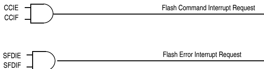
Figure 22-31. Flash Module Interrupts Implementation
