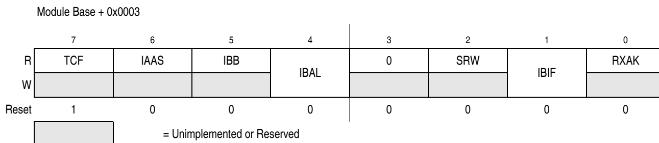
Figure 20-7. IIC Bus Status Register (IBSR)
