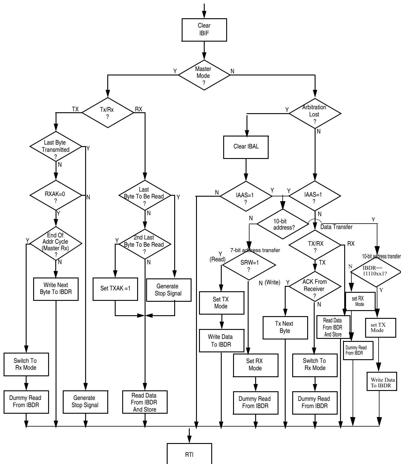
Figure 20-16. Flow-Chart of Typical IIC Interrupt Routine
